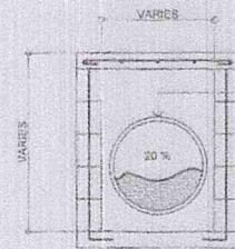
SECTION AT RCCP
