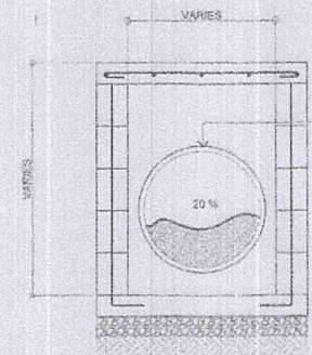
SECTION AT RCCP
