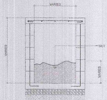
SECTION AT CHB
