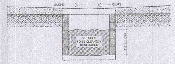
ROAD CROSS SECTION SCALE 1:200/475
